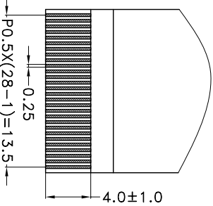
DETAIL DOTS SCALE: 10:1
